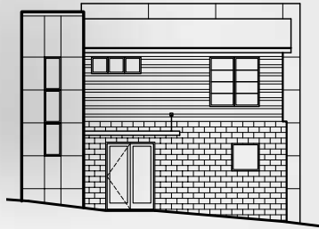
NORTH ELEVATION
